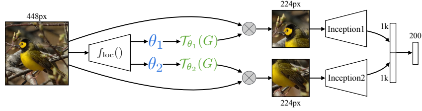
Figure 6: The architecture of the 2 \times \text{ST-CNN} 448px used for bird classification. A single localisation network f_{\text{loc}} predicts two transformation parameters \theta_1 and \theta_2 , with the subsequent transforms \mathcal{T}_{\theta_1} and \mathcal{T}_{\theta_2} applied to the original input image.
